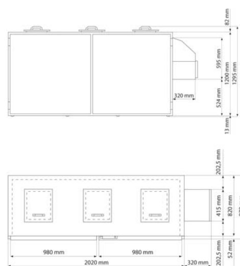
Waste disposal cooler 3 x 240 l
