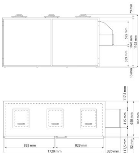
Waste disposal cooler 3 x 120 l
