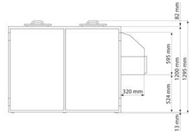
Waste disposal cooler 2 x 240 l
