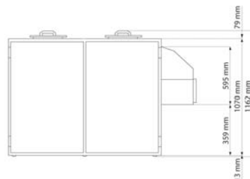
Waste disposal cooler 2 x 120 l
